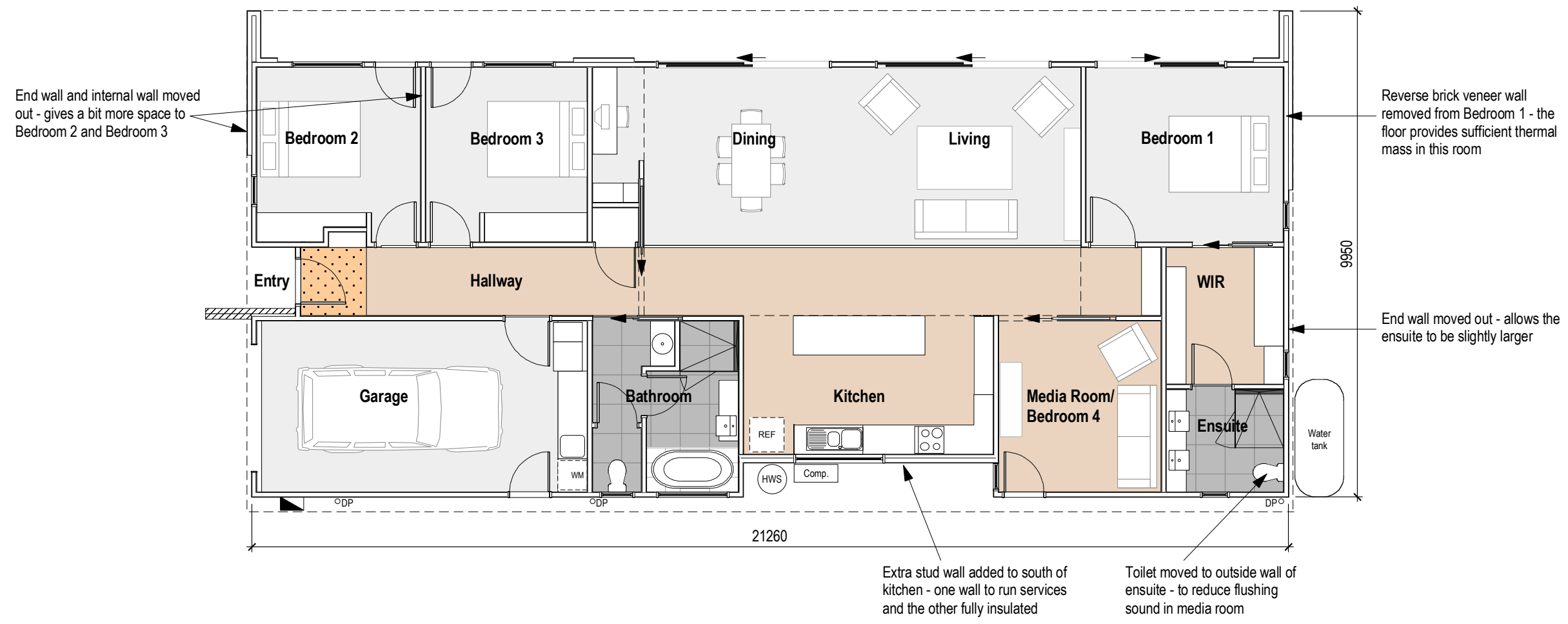
Energy Efficient Demonstration Home - Floor Plan: with changes if re-building Scale 1:100 on A3
